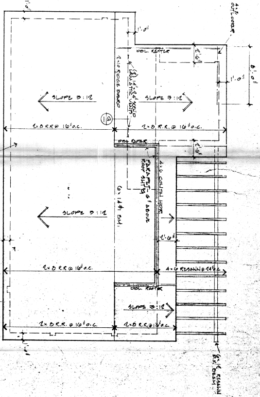
ROOF PLAN 1/4" = 1'-0"
